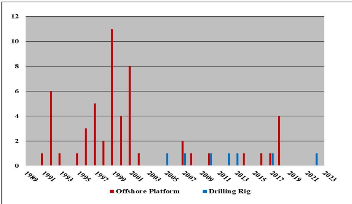
Figure 1: Number of Offshore Facility Incidents by Year and Facility Type (Excludes 2010 DEEPWATER HORIZON and TAYLOR ENERGY Oil Spills)
